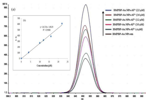
Figure 2 . (a) Fluorescence emission spectra of BMPBP-AuNPs after adding various concentration of \text{Al}^{3+} from 4 to 22 \mu\text{M} . (b) inset: the relationship between fluorescence intensity and \text{Al}^{3+} concentration.
