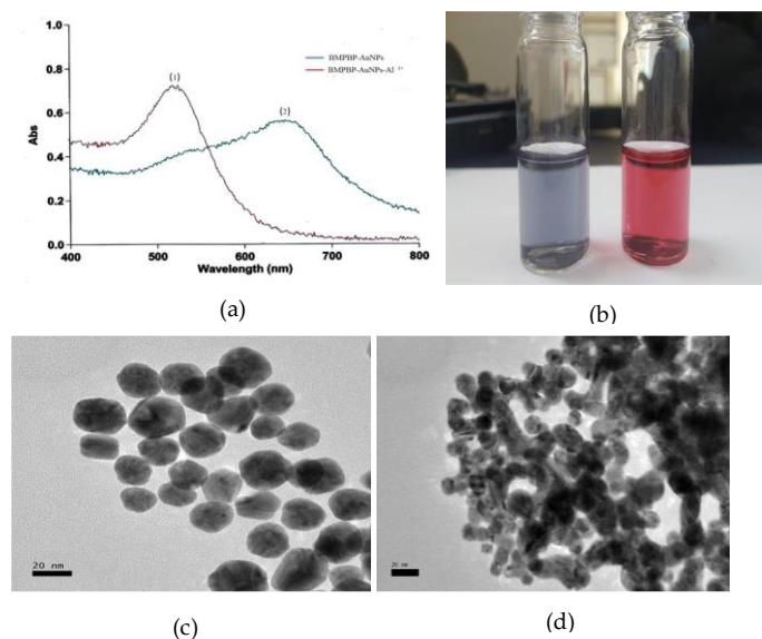
Figure 1. Absorption spectra (a), Optical photographs (b) of BMPBP-AuNPs without and with \text{Al}^{3+} (5.7Mm). TEM image (c) BMPBP-AuNPs (d) TEM image of BMPBP-AuNPs- \text{Al}^{3+} .
