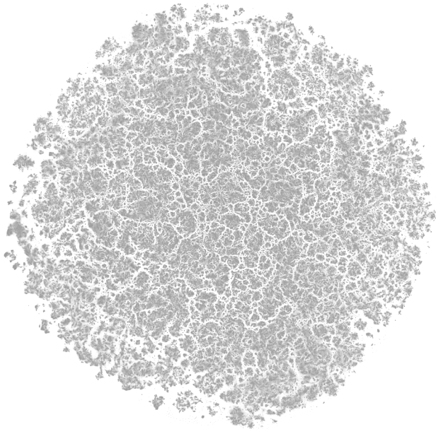
a BERT
