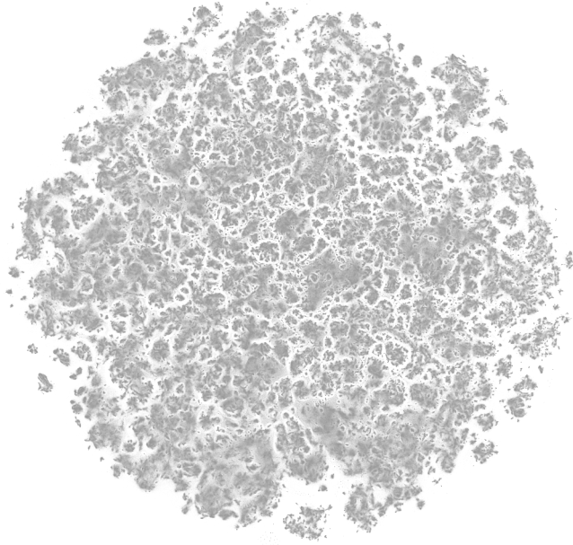
b TF-IDF
