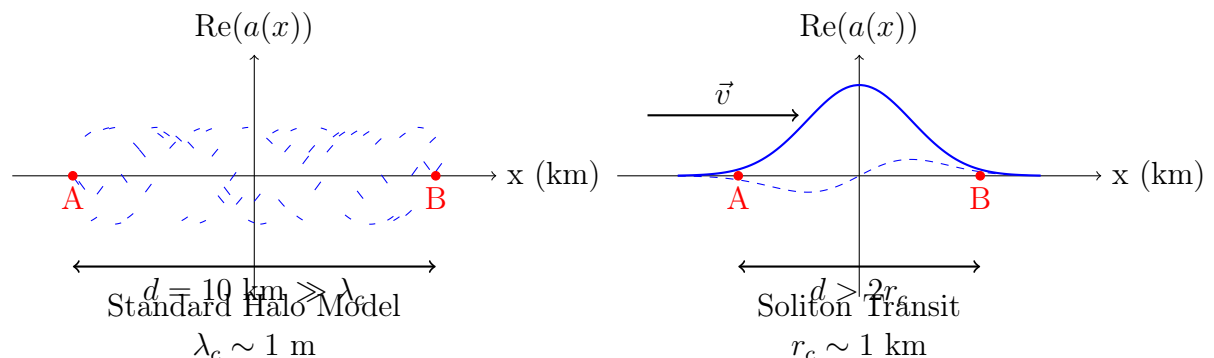
Figure 1: Conceptual contrast of field coherence. (Left) Stochastic SHM field: detectors A and B sample uncorrelated phases. (Right) A coherent soliton envelope transits the baseline, imposing correlated amplitude/phase modulation on both detectors.
